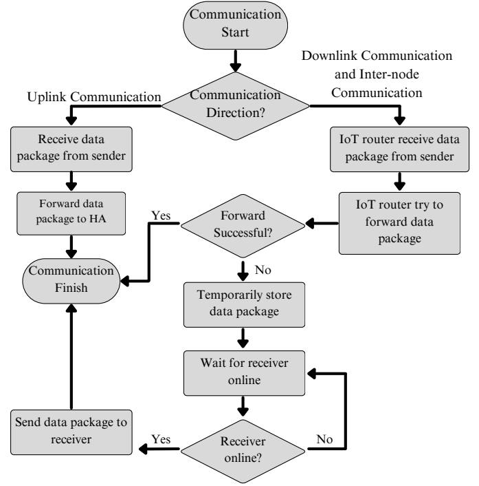
Fig. 2. Communication flowchart.
